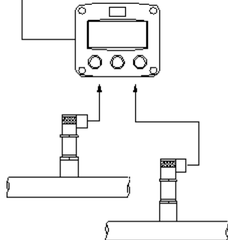
RS232/RS485 Modbus (option)
